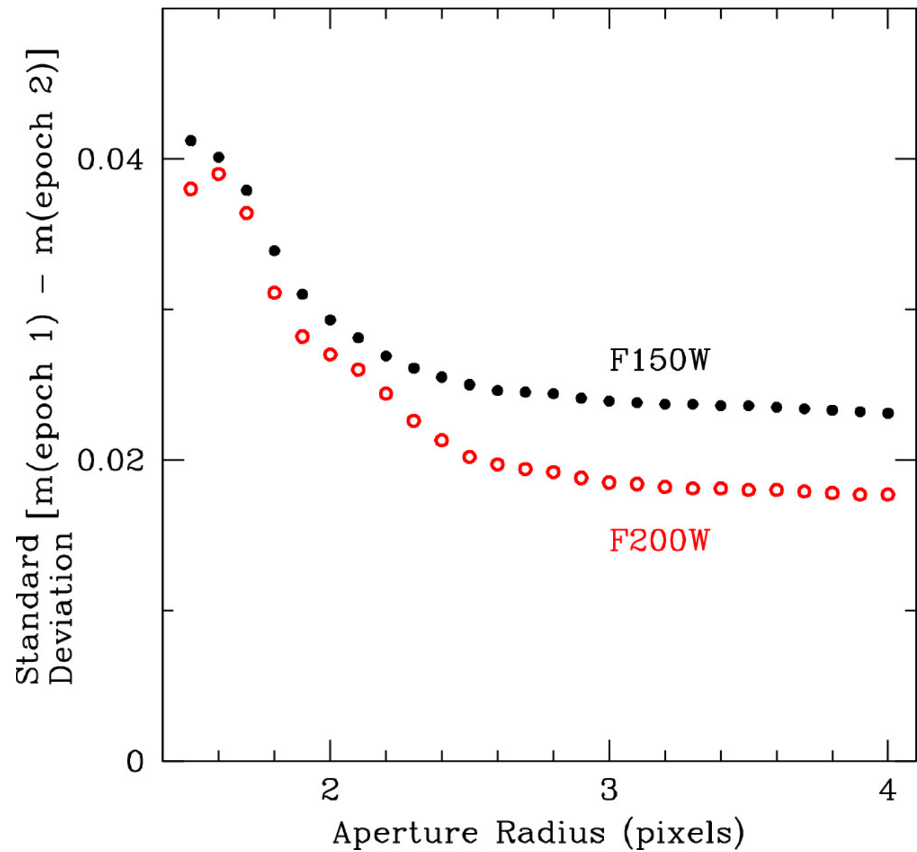
Figure 1. from K. L. Luhman 2024 Astron. J. 168 doi:10.3847/1538-3881/ad812a https://dx.doi.org/10.3847/1538-3881/ad812a © 2024. The Author(s). Published by the American Astronomical Society.
