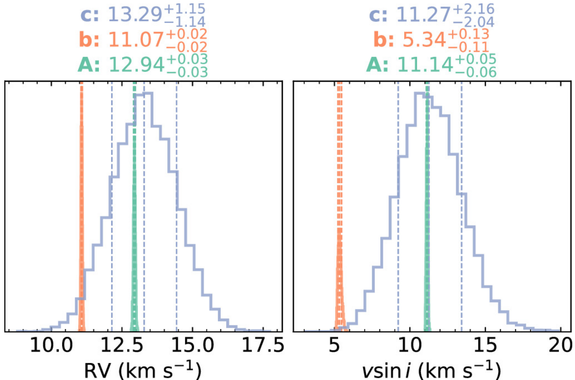
Figure 9. from Yapeng Zhang et al 2024 Astron. J. 168 doi:10.3847/1538-3881/ad7ea9 https://dx.doi.org/10.3847/1538-3881/ad7ea9 © 2024. The Author(s). Published by the American Astronomical Society.
