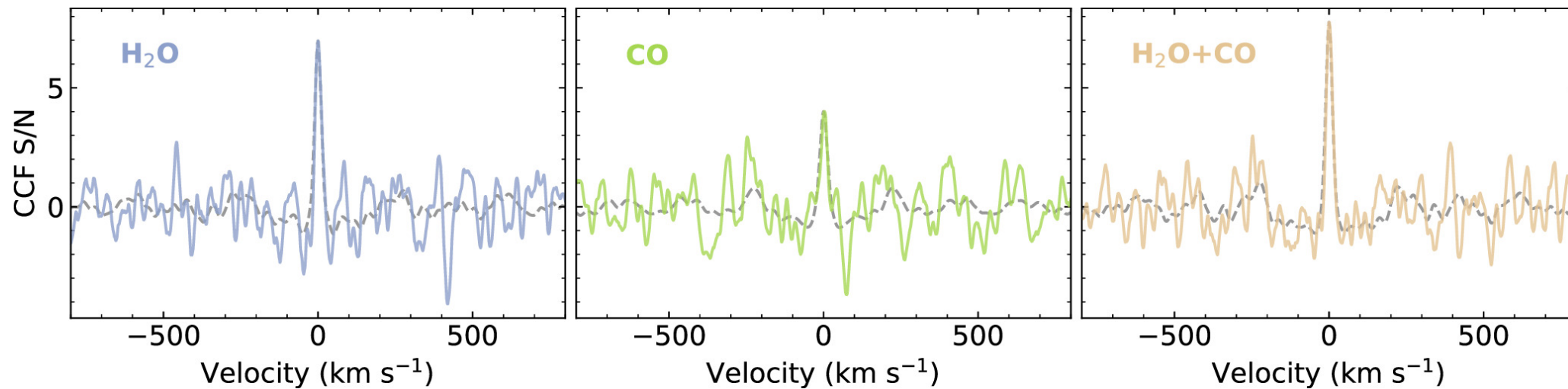
Figure 6. from Yapeng Zhang et al 2024 Astron. J. 168 doi:10.3847/1538-3881/ad7ea9 https://dx.doi.org/10.3847/1538-3881/ad7ea9 © 2024. The Author(s). Published by the American Astronomical Society.
