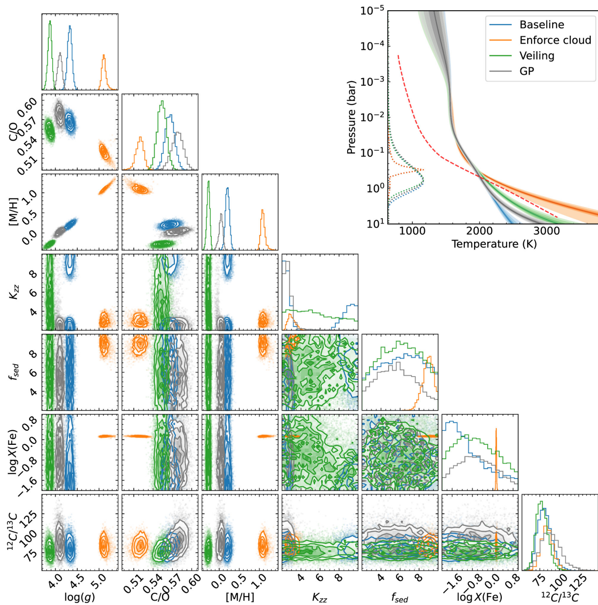
Figure 5. from Yapeng Zhang et al 2024 Astron. J. 168 doi:10.3847/1538-3881/ad7ea9 https://dx.doi.org/10.3847/1538-3881/ad7ea9 © 2024. The Author(s). Published by the American Astronomical Society.
