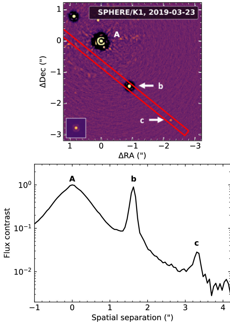
Figure 1. from Yapeng Zhang et al 2024 Astron. J. 168 doi:10.3847/1538-3881/ad7ea9 https://dx.doi.org/10.3847/1538-3881/ad7ea9 © 2024. The Author(s). Published by the American Astronomical Society.
