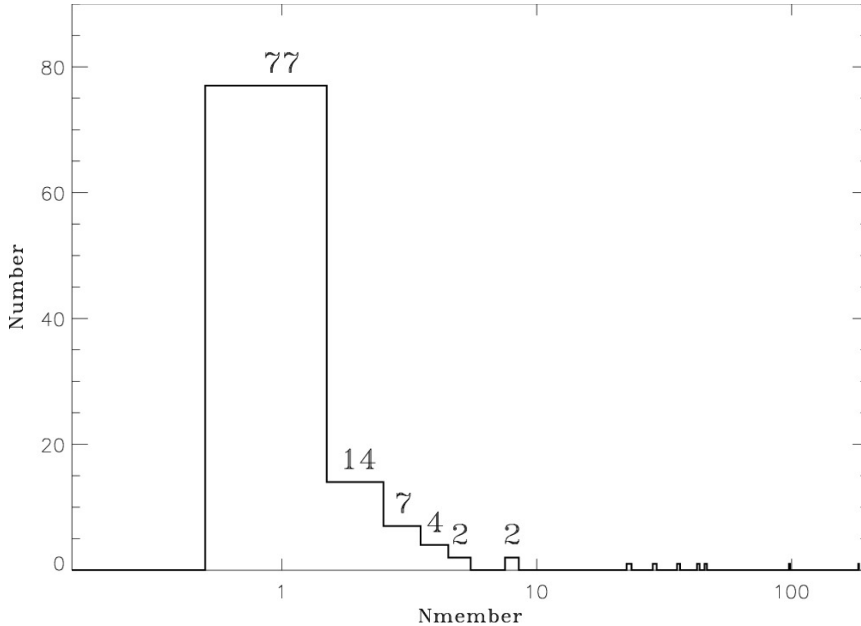
Figure 8. from Yu-zhong Wu and Wei Zhang 2024 Astron. J. 168 doi:10.3847/1538-3881/ad7e1e https://dx.doi.org/10.3847/1538-3881/ad7e1e © 2024. The Author(s). Published by the American Astronomical Society.
