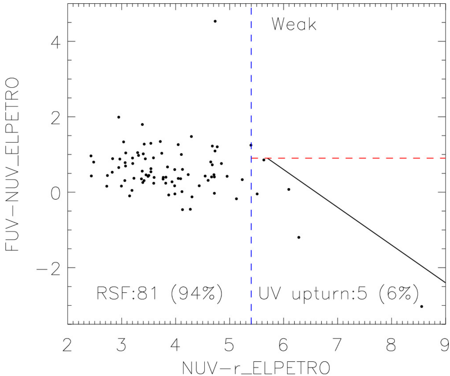
Figure 6. from Yu-zhong Wu and Wei Zhang 2024 Astron. J. 168 doi:10.3847/1538-3881/ad7e1e https://dx.doi.org/10.3847/1538-3881/ad7e1e © 2024. The Author(s). Published by the American Astronomical Society.
