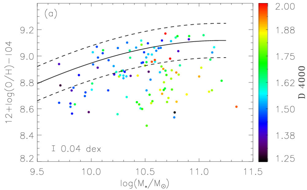
Figure 5. from Yu-zhong Wu and Wei Zhang 2024 Astron. J. 168 doi:10.3847/1538-3881/ad7e1e https://dx.doi.org/10.3847/1538-3881/ad7e1e © 2024. The Author(s). Published by the American Astronomical Society.
