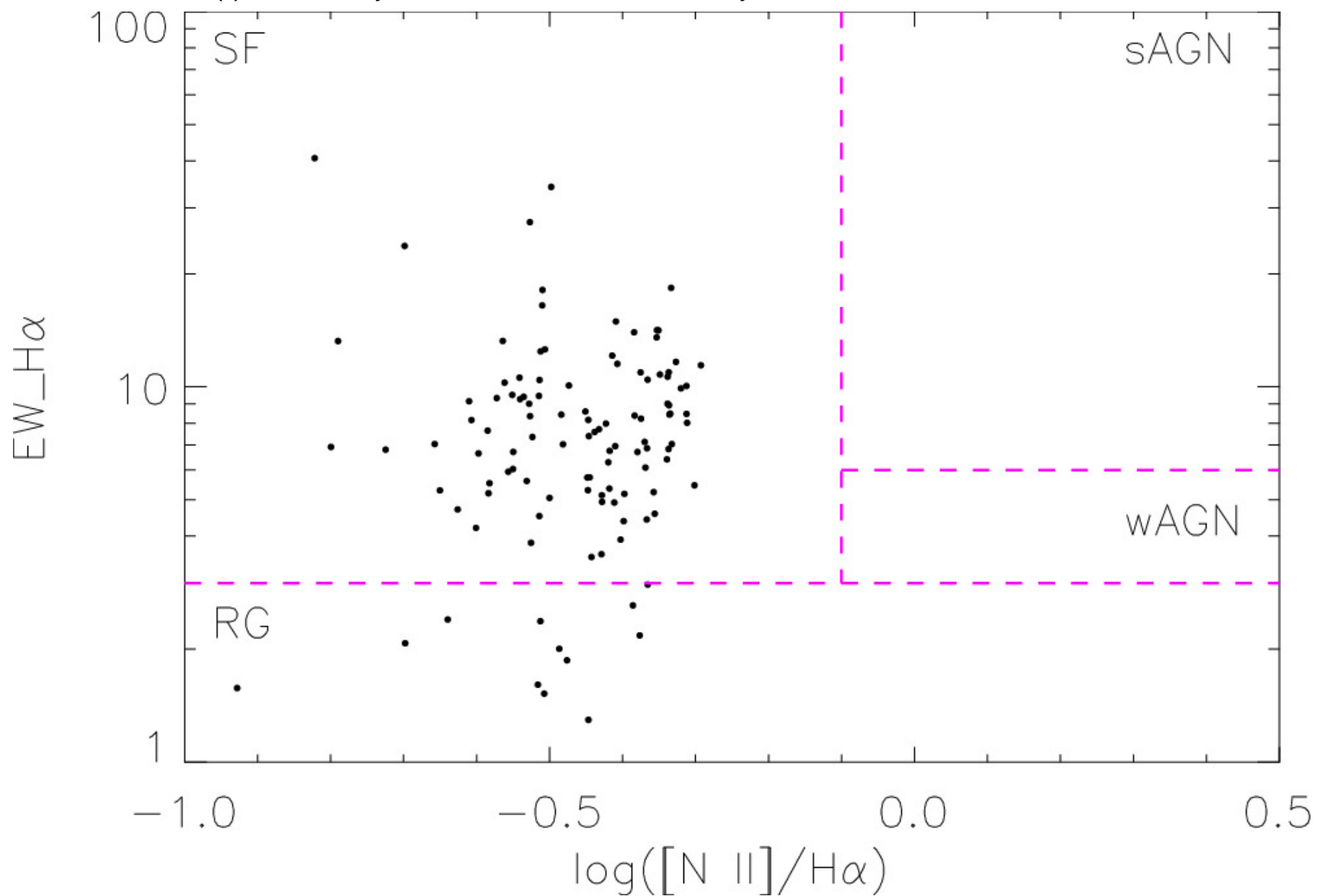
Figure 4. from Yu-zhong Wu and Wei Zhang 2024 Astron. J. 168 doi:10.3847/1538-3881/ad7e1e https://dx.doi.org/10.3847/1538-3881/ad7e1e © 2024. The Author(s). Published by the American Astronomical Society.
