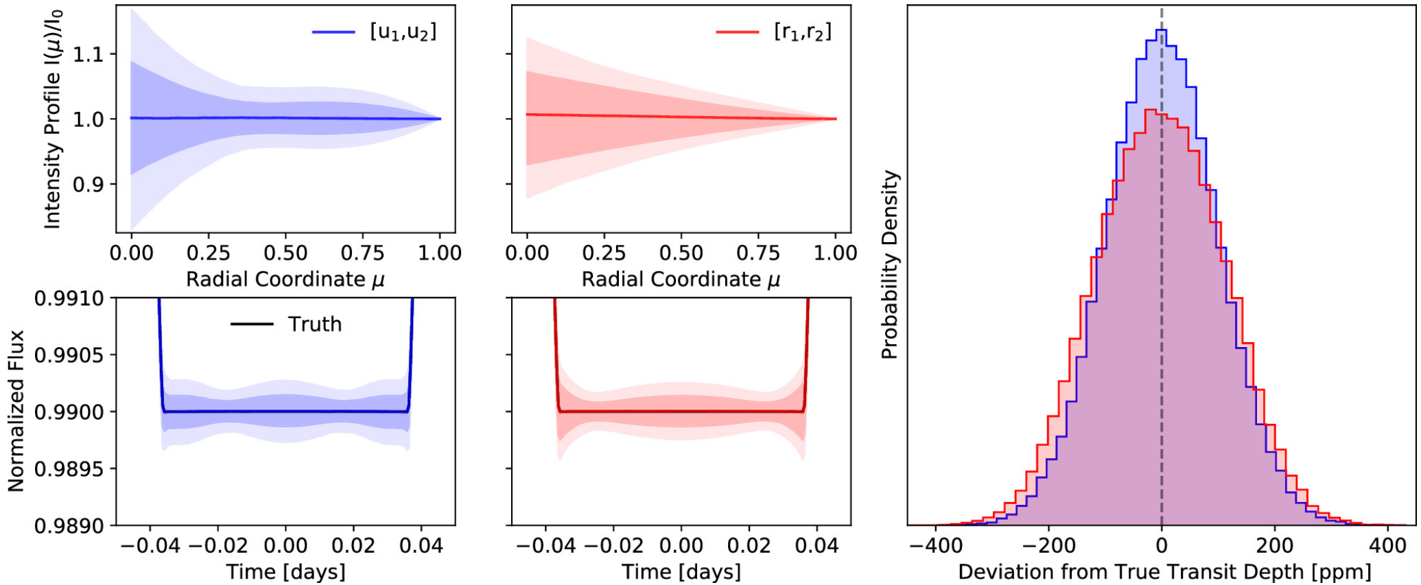
Figure 6. from Louis-Philippe Coulombe et al 2024 Astron. J. 168 doi:10.3847/1538-3881/ad7aef https://dx.doi.org/10.3847/1538-3881/ad7aef © 2024. The Author(s). Published by the American Astronomical Society.
