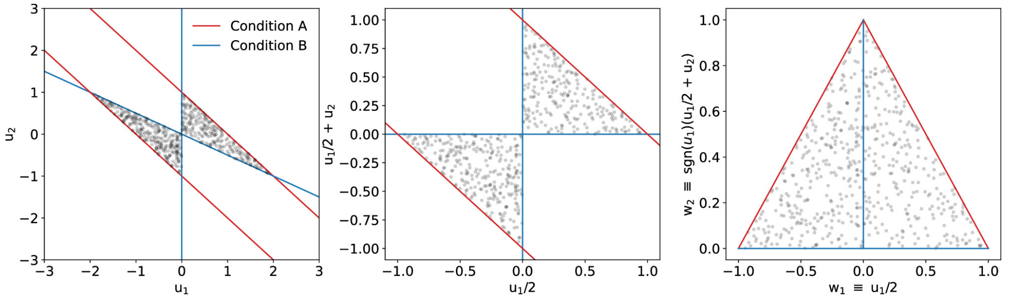
Figure 5. from Louis-Philippe Coulombe et al 2024 Astron. J. 168 doi:10.3847/1538-3881/ad7aef https://dx.doi.org/10.3847/1538-3881/ad7aef © 2024. The Author(s). Published by the American Astronomical Society.
