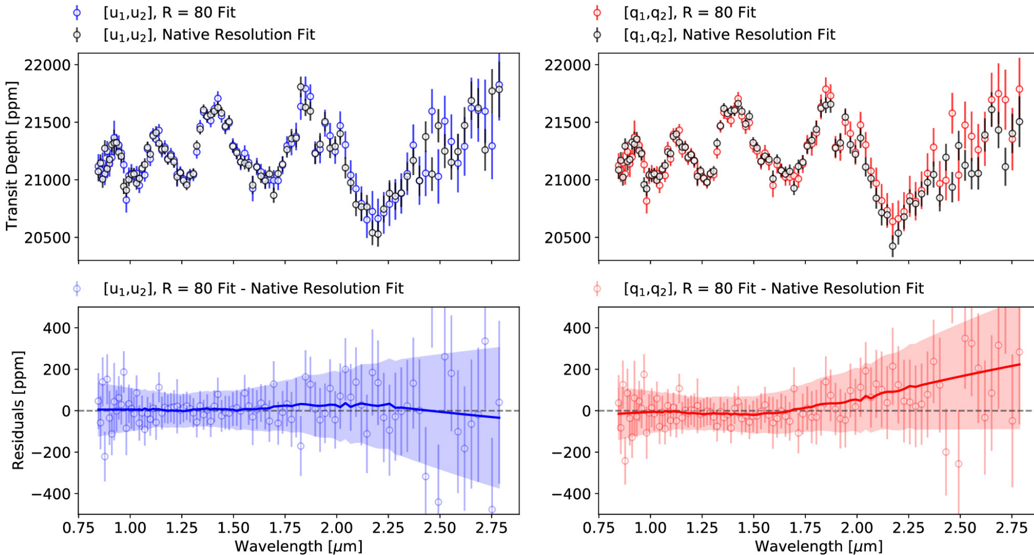
Figure 3. from Louis-Philippe Coulombe et al 2024 Astron. J. 168 doi:10.3847/1538-3881/ad7aef https://dx.doi.org/10.3847/1538-3881/ad7aef
