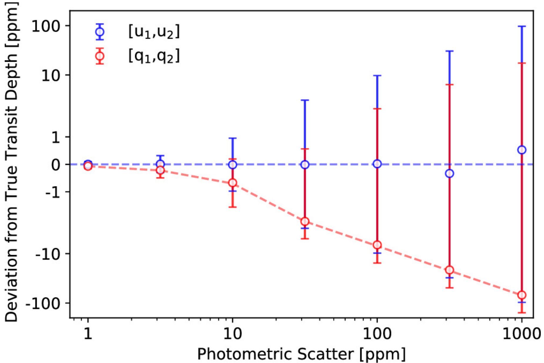
Figure 2. from Louis-Philippe Coulombe et al 2024 Astron. J. 168 doi:10.3847/1538-3881/ad7aef https://dx.doi.org/10.3847/1538-3881/ad7aef © 2024. The Author(s). Published by the American Astronomical Society.
