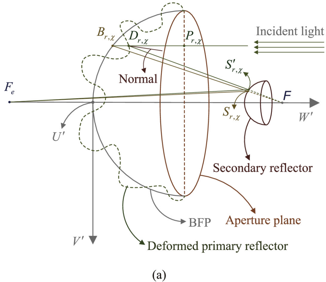
Figure 3. from Jia You and Zheng Wang 2024 Astron. J. 168 doi:10.3847/1538-3881/ad7376 https://dx.doi.org/10.3847/1538-3881/ad7376 © 2024. The Author(s). Published by the American Astronomical Society.
