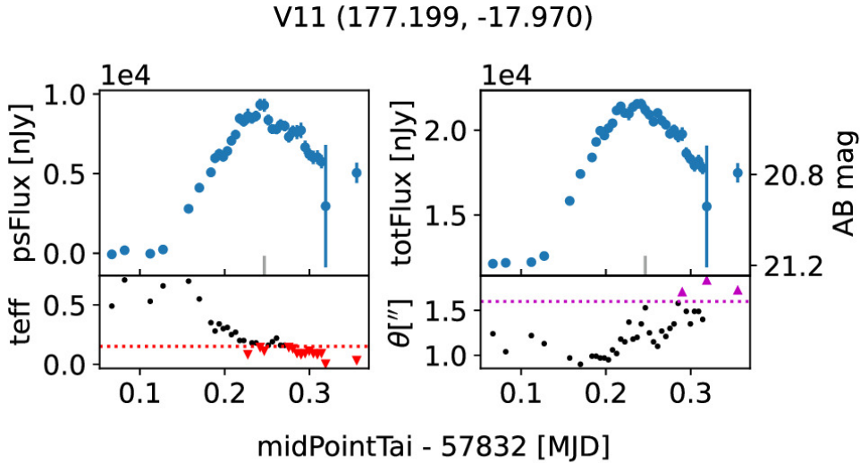
Figure 9. from Shenming Fu et al 2024 Astron. J. 168 doi:10.3847/1538-3881/ad70b1 https://dx.doi.org/10.3847/1538-3881/ad70b1 © 2024. The Author(s). Published by the American Astronomical Society.
