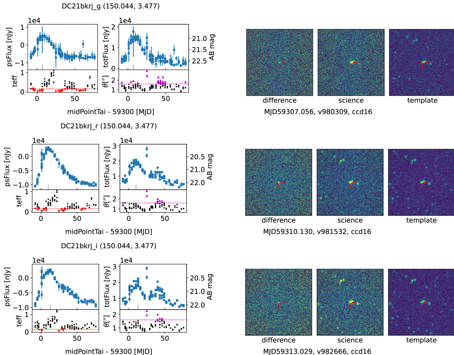
Figure 7. from Shenming Fu et al 2024 Astron. J. 168 doi:10.3847/1538-3881/ad70b1 https://dx.doi.org/10.3847/1538-3881/ad70b1 © 2024. The Author(s). Published by the American Astronomical Society.
