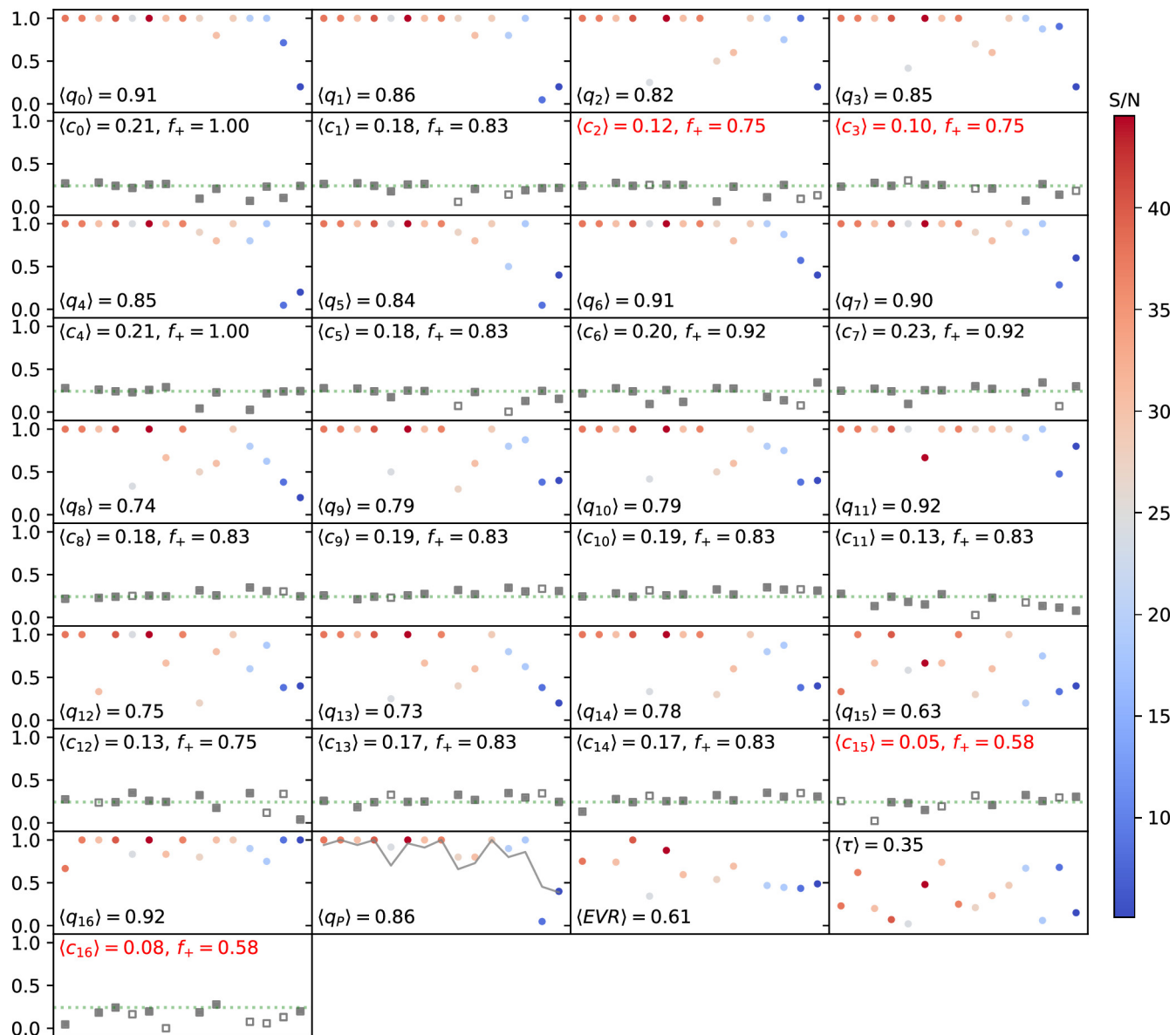
Figure 24. from Shenming Fu et al 2024 Astron. J. 168 doi:10.3847/1538-3881/ad70b1 https://dx.doi.org/10.3847/1538-3881/ad70b1 © 2024. The Author(s). Published by the American Astronomical Society.
