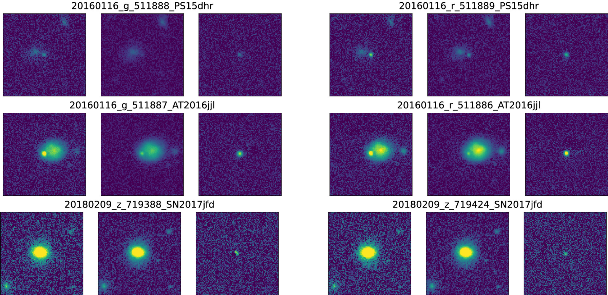
Figure 22. from Shenming Fu et al 2024 Astron. J. 168 doi:10.3847/1538-3881/ad70b1 https://dx.doi.org/10.3847/1538-3881/ad70b1 © 2024. The Author(s). Published by the American Astronomical Society.
