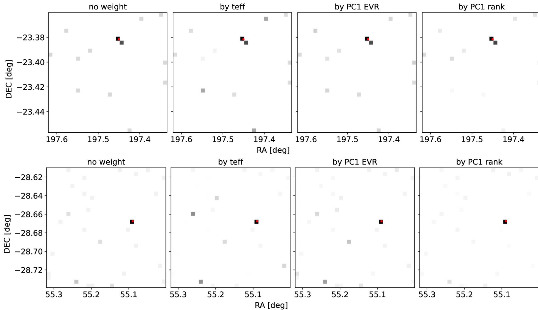
Figure 21. from Shenming Fu et al 2024 Astron. J. 168 doi:10.3847/1538-3881/ad70b1 https://dx.doi.org/10.3847/1538-3881/ad70b1 © 2024. The Author(s). Published by the American Astronomical Society.
