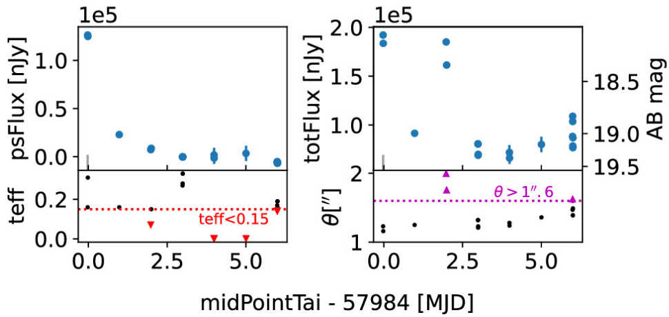
Figure 2. from Shenming Fu et al 2024 Astron. J. 168 doi:10.3847/1538-3881/ad70b1 https://dx.doi.org/10.3847/1538-3881/ad70b1 © 2024. The Author(s). Published by the American Astronomical Society. GW170817_g (197.450, -23.382)
