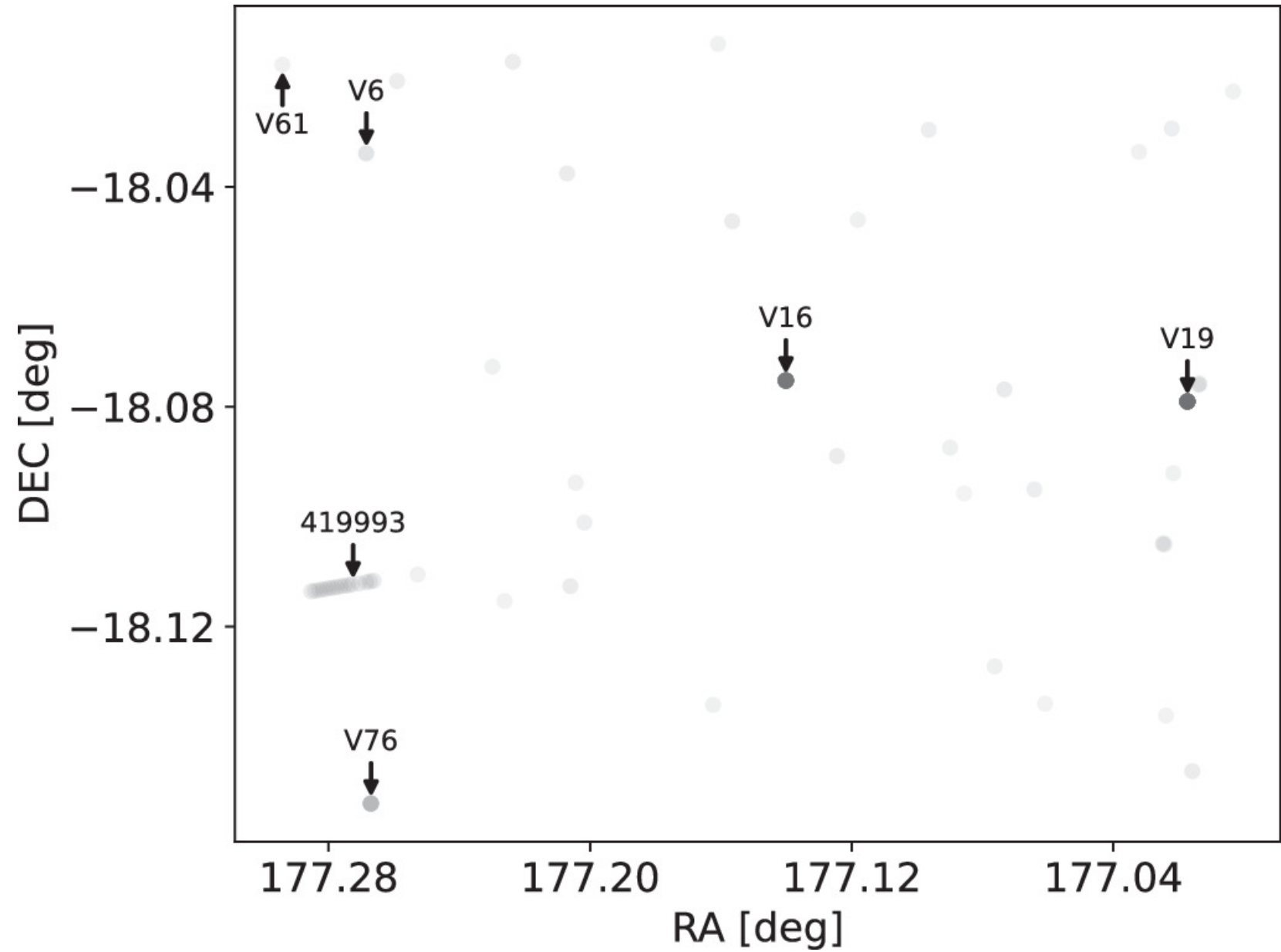
Figure 19. from Shenming Fu et al 2024 Astron. J. 168 doi:10.3847/1538-3881/ad70b1 https://dx.doi.org/10.3847/1538-3881/ad70b1 © 2024. The Author(s). Published by the American Astronomical Society.
