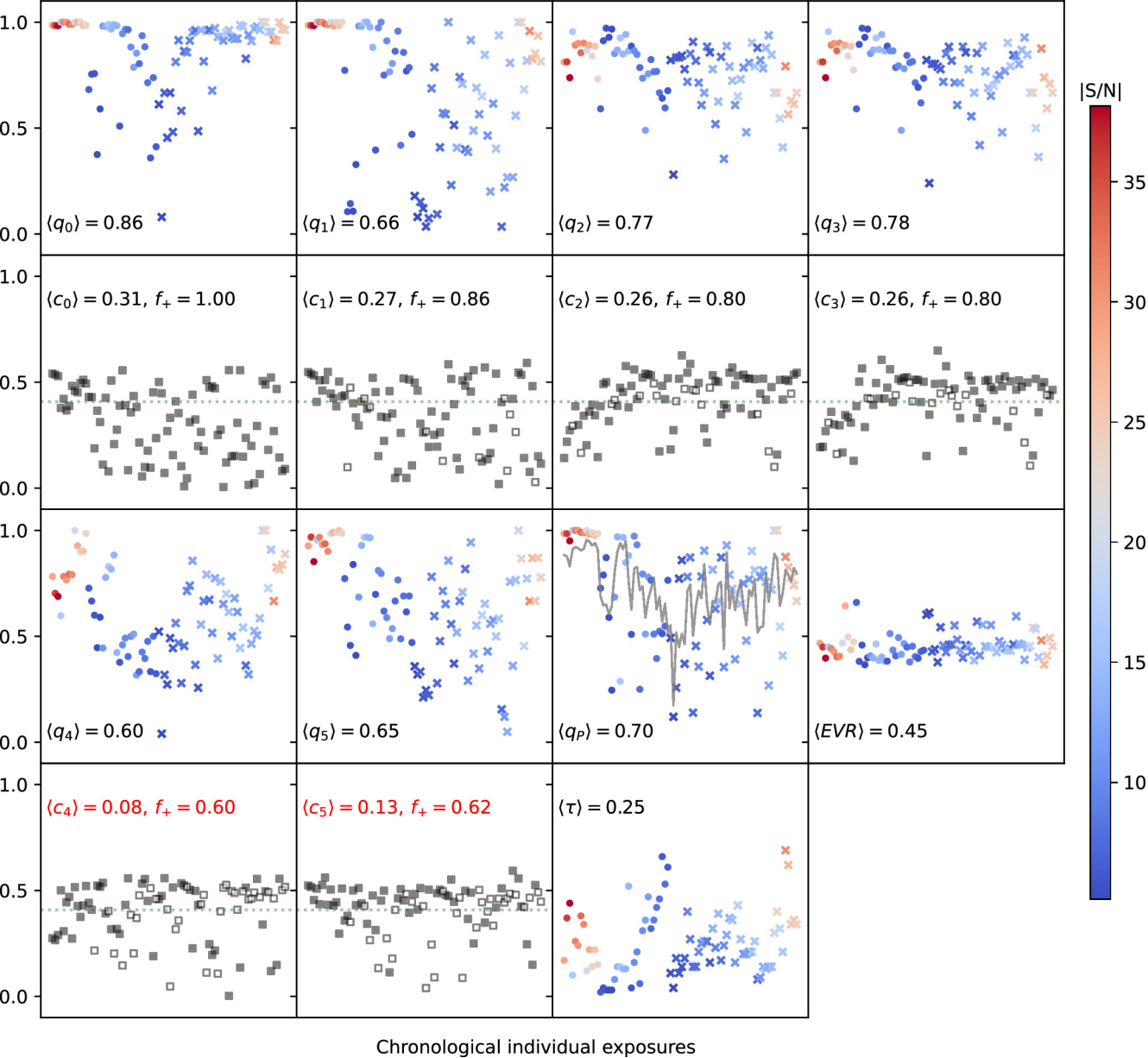
Figure 17. from Shenming Fu et al 2024 Astron. J. 168 doi:10.3847/1538-3881/ad70b1 https://dx.doi.org/10.3847/1538-3881/ad70b1 © 2024. The Author(s). Published by the American Astronomical Society.
