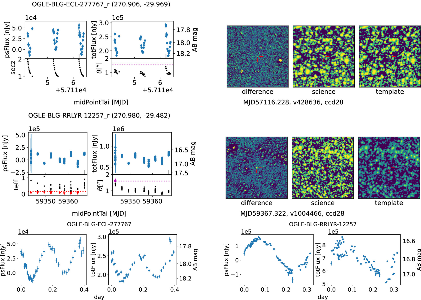
Figure 10. from Shenming Fu et al 2024 Astron. J. 168 doi:10.3847/1538-3881/ad70b1 https://dx.doi.org/10.3847/1538-3881/ad70b1 © 2024. The Author(s). Published by the American Astronomical Society.
