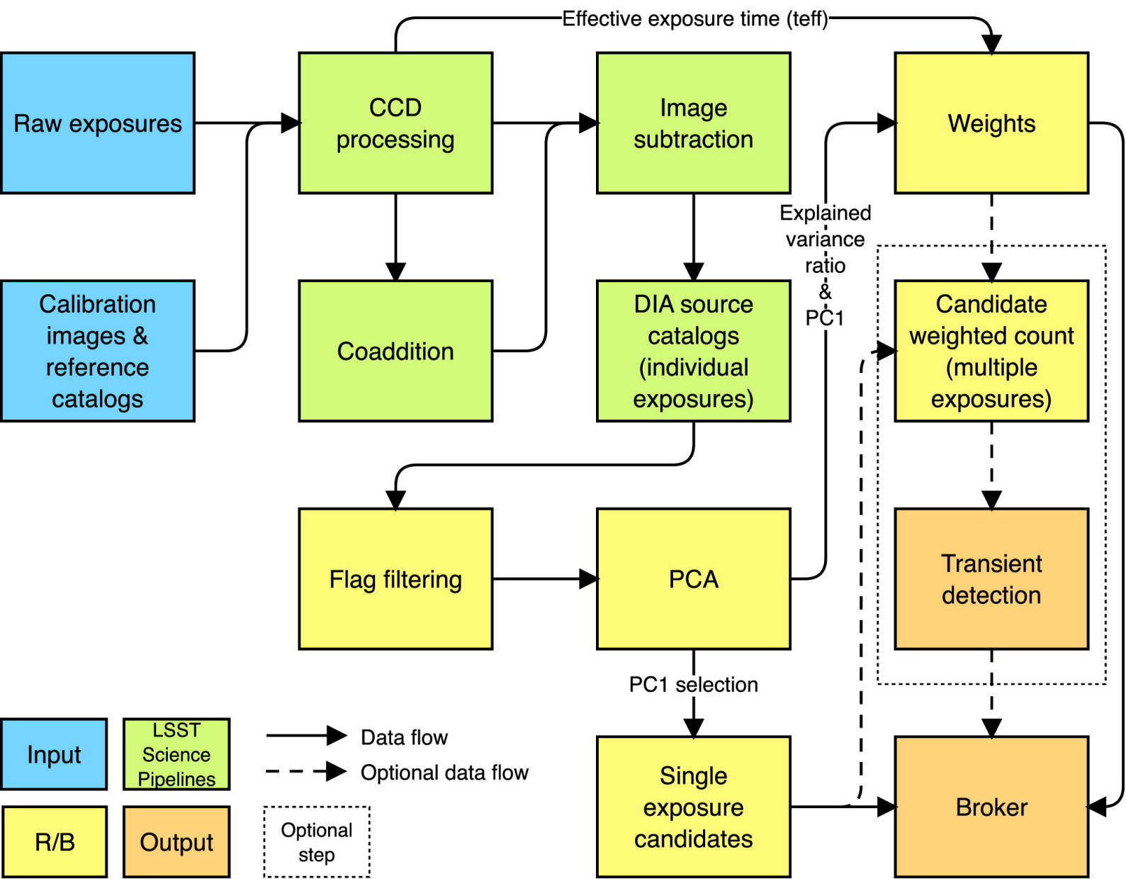
Figure 1. from Shenming Fu et al 2024 Astron. J. 168 doi:10.3847/1538-3881/ad70b1 https://dx.doi.org/10.3847/1538-3881/ad70b1 © 2024. The Author(s). Published by the American Astronomical Society.
