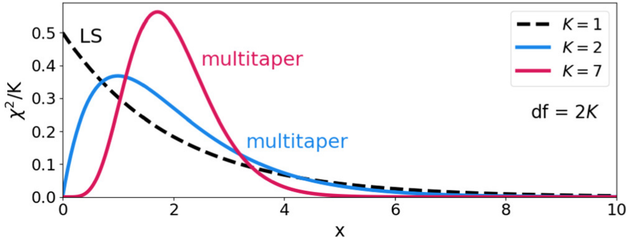
Figure 8. from Aarya A. Patil et al 2024 Astron. J. 168 doi:10.3847/1538-3881/ad7029 https://dx.doi.org/10.3847/1538-3881/ad7029 © 2024. The Author(s). Published by the American Astronomical Society.
