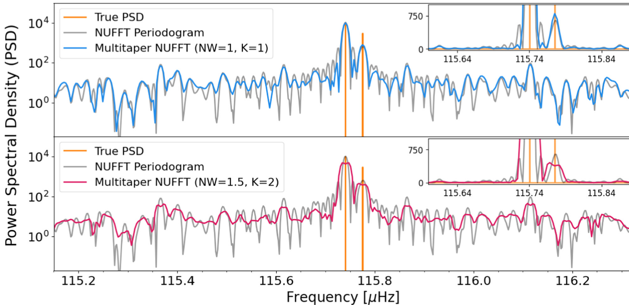
Figure 6. from Aarya A. Patil et al 2024 Astron. J. 168 doi:10.3847/1538-3881/ad7029 https://dx.doi.org/10.3847/1538-3881/ad7029 © 2024. The Author(s). Published by the American Astronomical Society.
