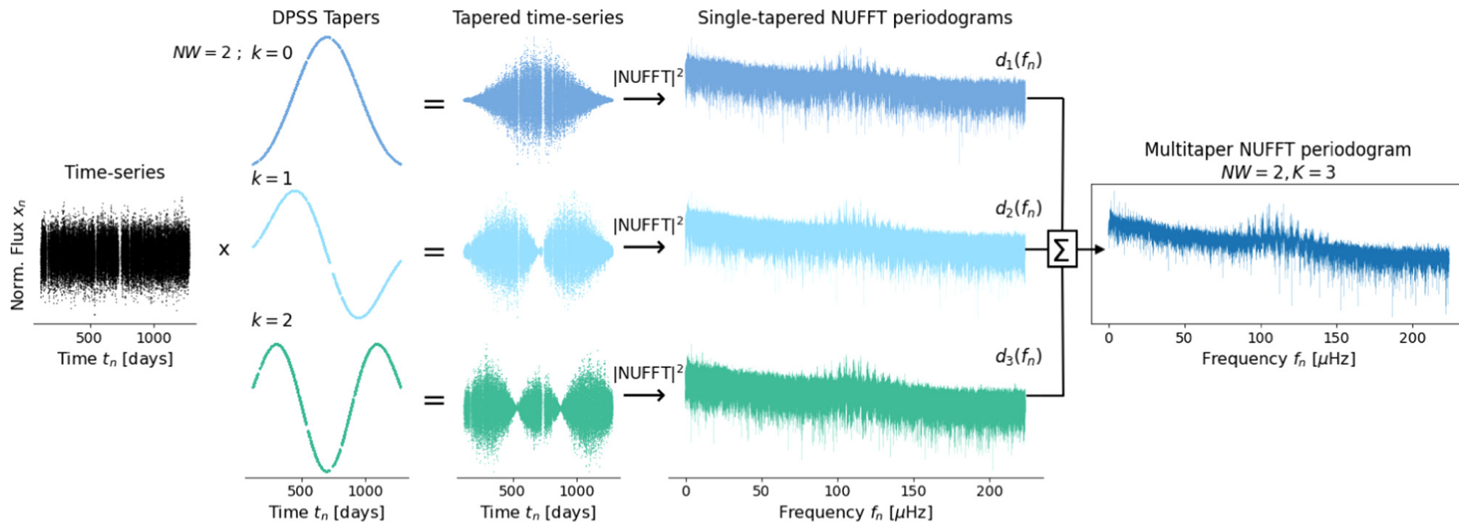
Figure 4. from Aarya A. Patil et al 2024 Astron. J. 168 doi:10.3847/1538-3881/ad7029 https://dx.doi.org/10.3847/1538-3881/ad7029 © 2024. The Author(s). Published by the American Astronomical Society.
