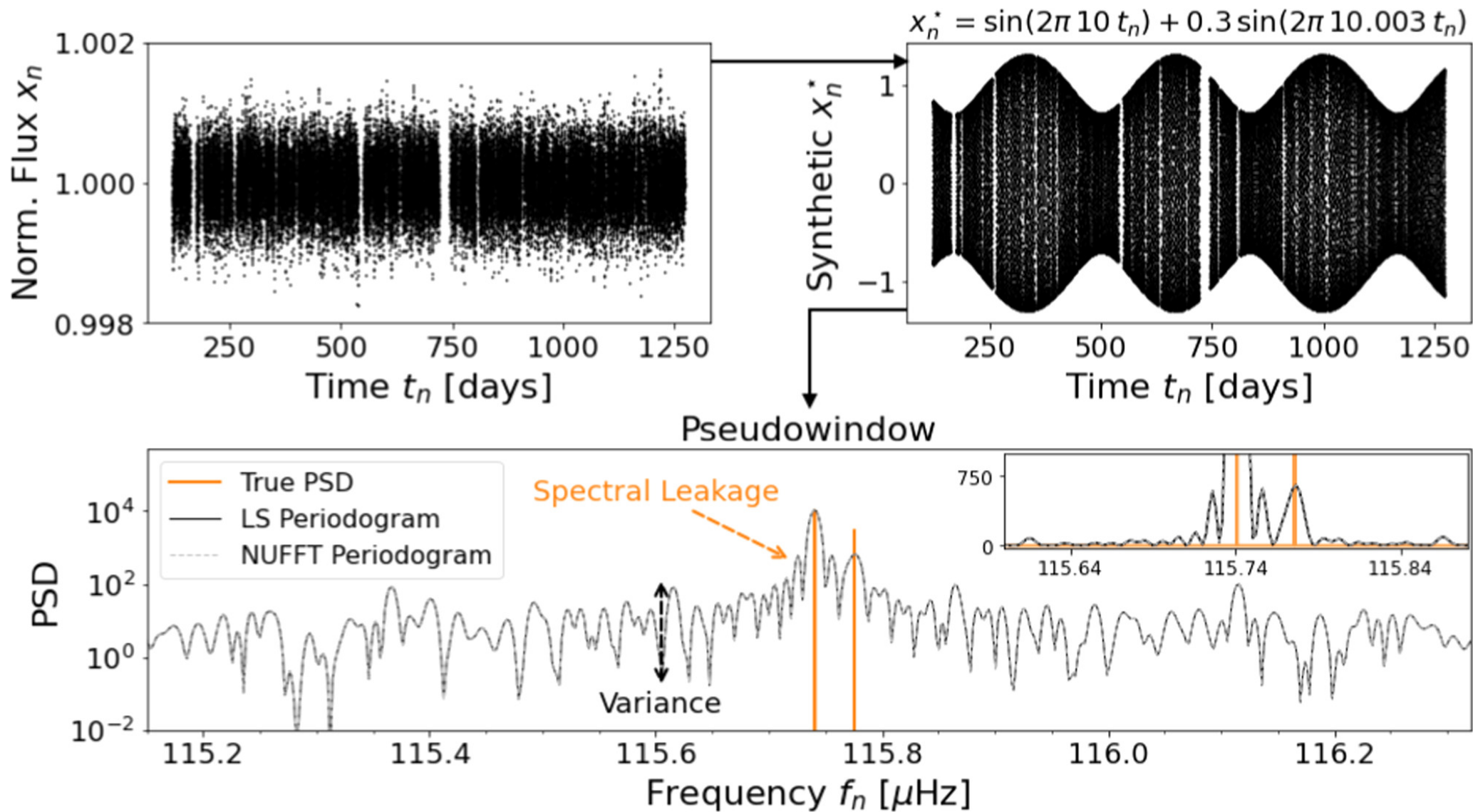
Figure 3. from Aarya A. Patil et al 2024 Astron. J. 168 doi:10.3847/1538-3881/ad7029 https://dx.doi.org/10.3847/1538-3881/ad7029 © 2024. The Author(s). Published by the American Astronomical Society.
