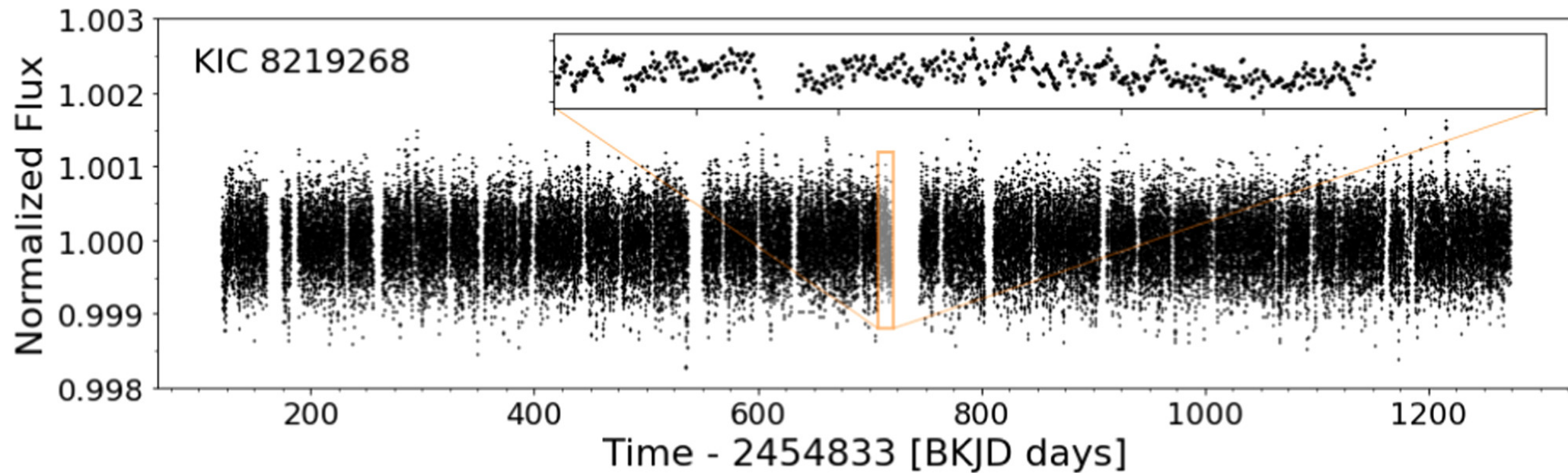
Figure 1. from Aarya A. Patil et al 2024 Astron. J. 168 doi:10.3847/1538-3881/ad7029 https://dx.doi.org/10.3847/1538-3881/ad7029 © 2024. The Author(s). Published by the American Astronomical Society.
