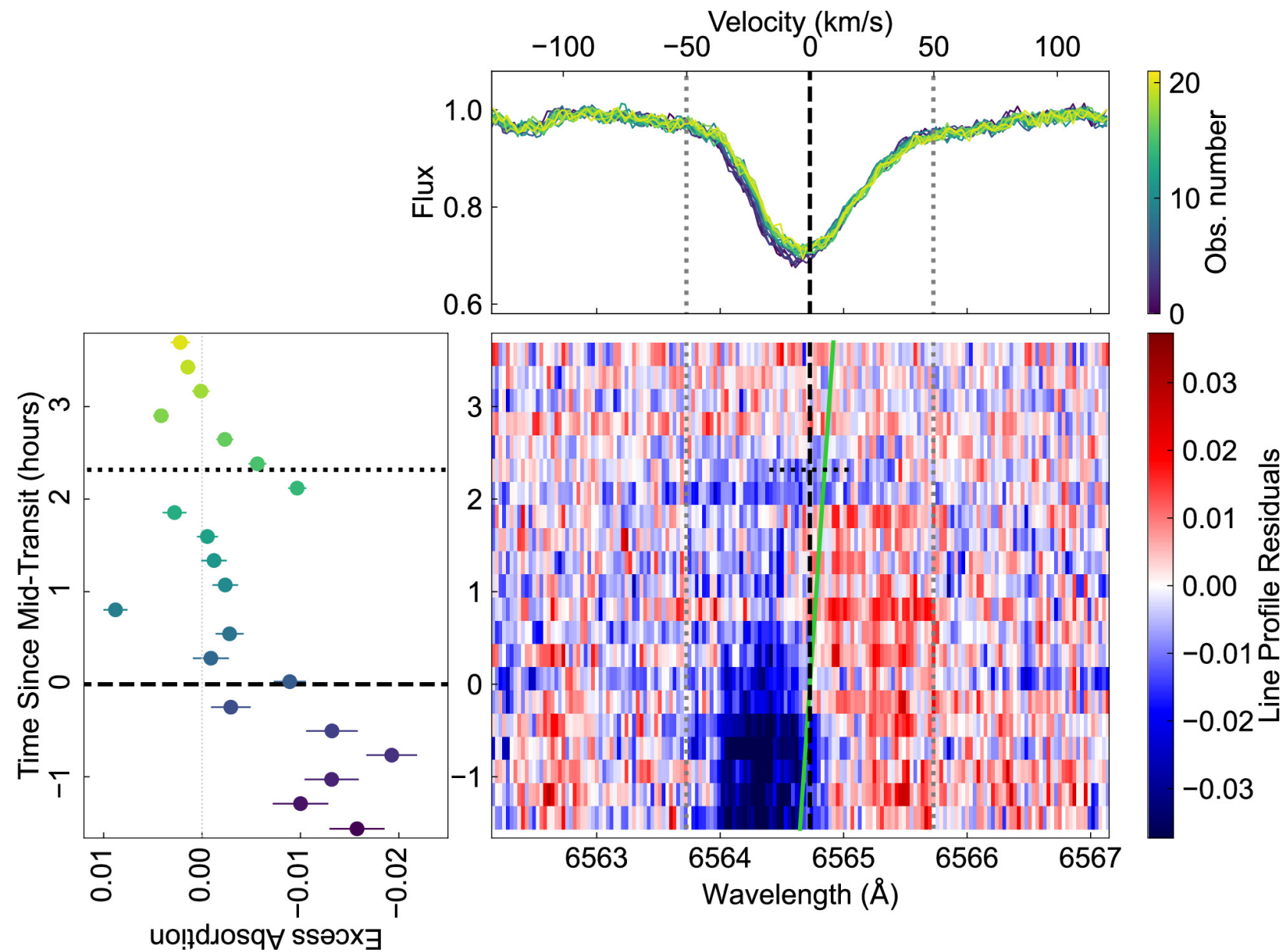
Figure 3. from Huan-Yu Teng et al 2024 Astron. J. 168 doi:10.3847/1538-3881/ad7022 https://dx.doi.org/10.3847/1538-3881/ad7022 © 2024. The Author(s). Published by the American Astronomical Society.
