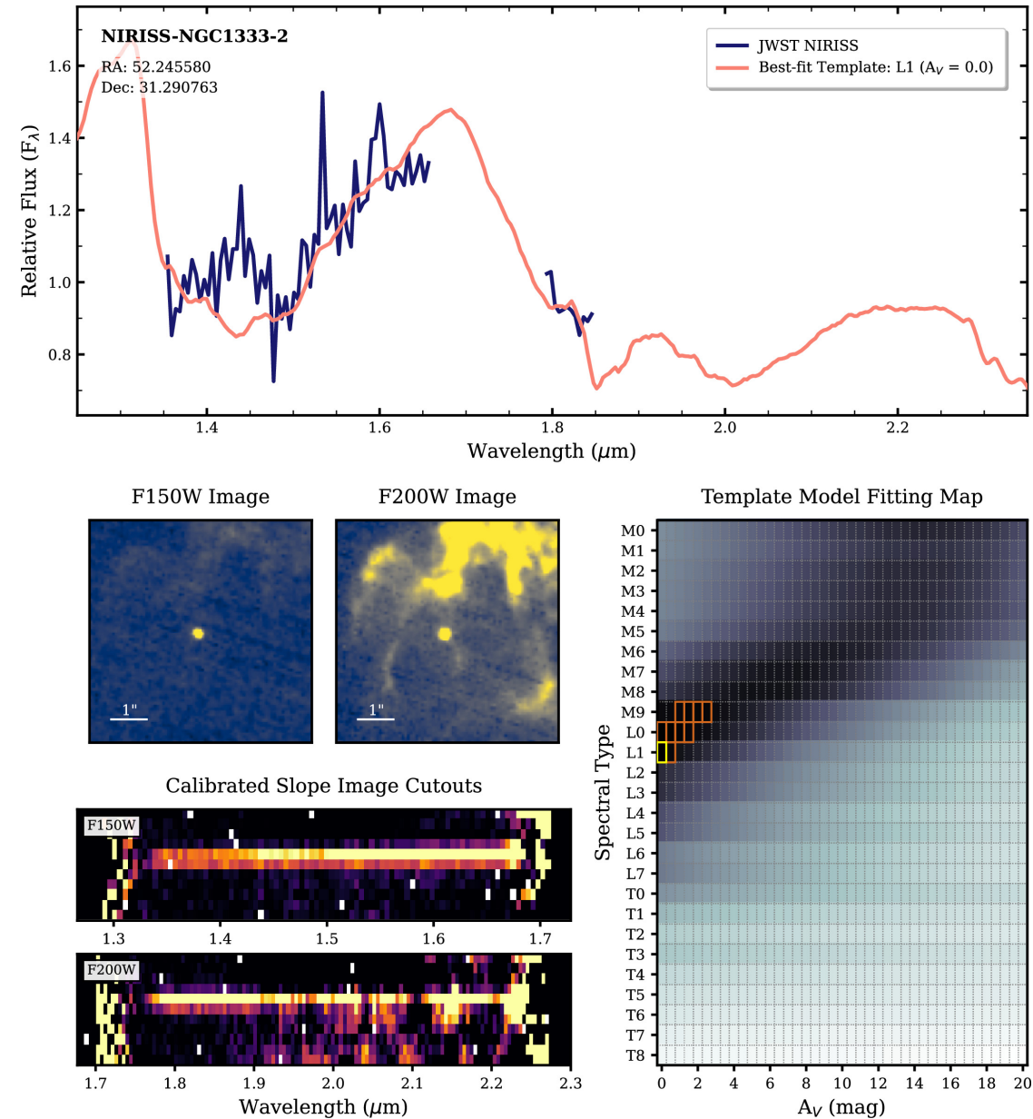
Figure 9. from Adam B. Langeveld et al 2024 Astron. J. 168 doi:10.3847/1538-3881/ad6f0c https://dx.doi.org/10.3847/1538-3881/ad6f0c © 2024. The Author(s). Published by the American Astronomical Society.
