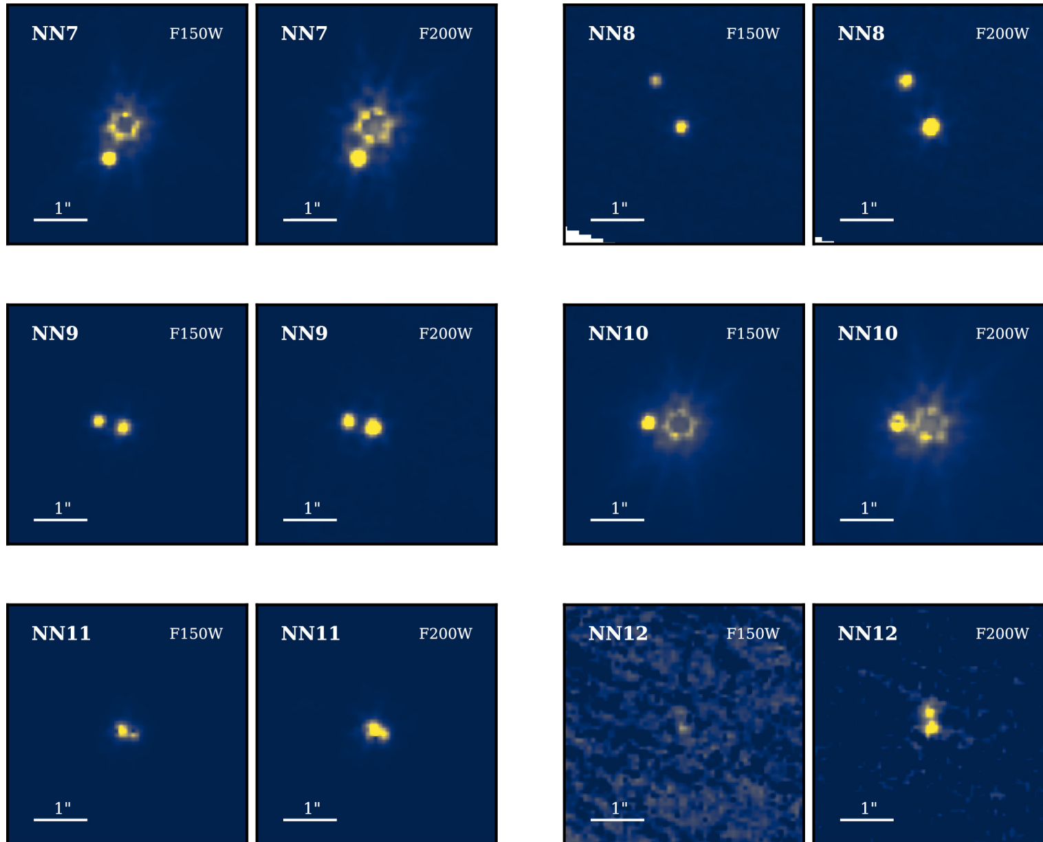
Figure 8. from Adam B. Langeveld et al 2024 Astron. J. 168 doi:10.3847/1538-3881/ad6f0c https://dx.doi.org/10.3847/1538-3881/ad6f0c © 2024. The Author(s). Published by the American Astronomical Society.
