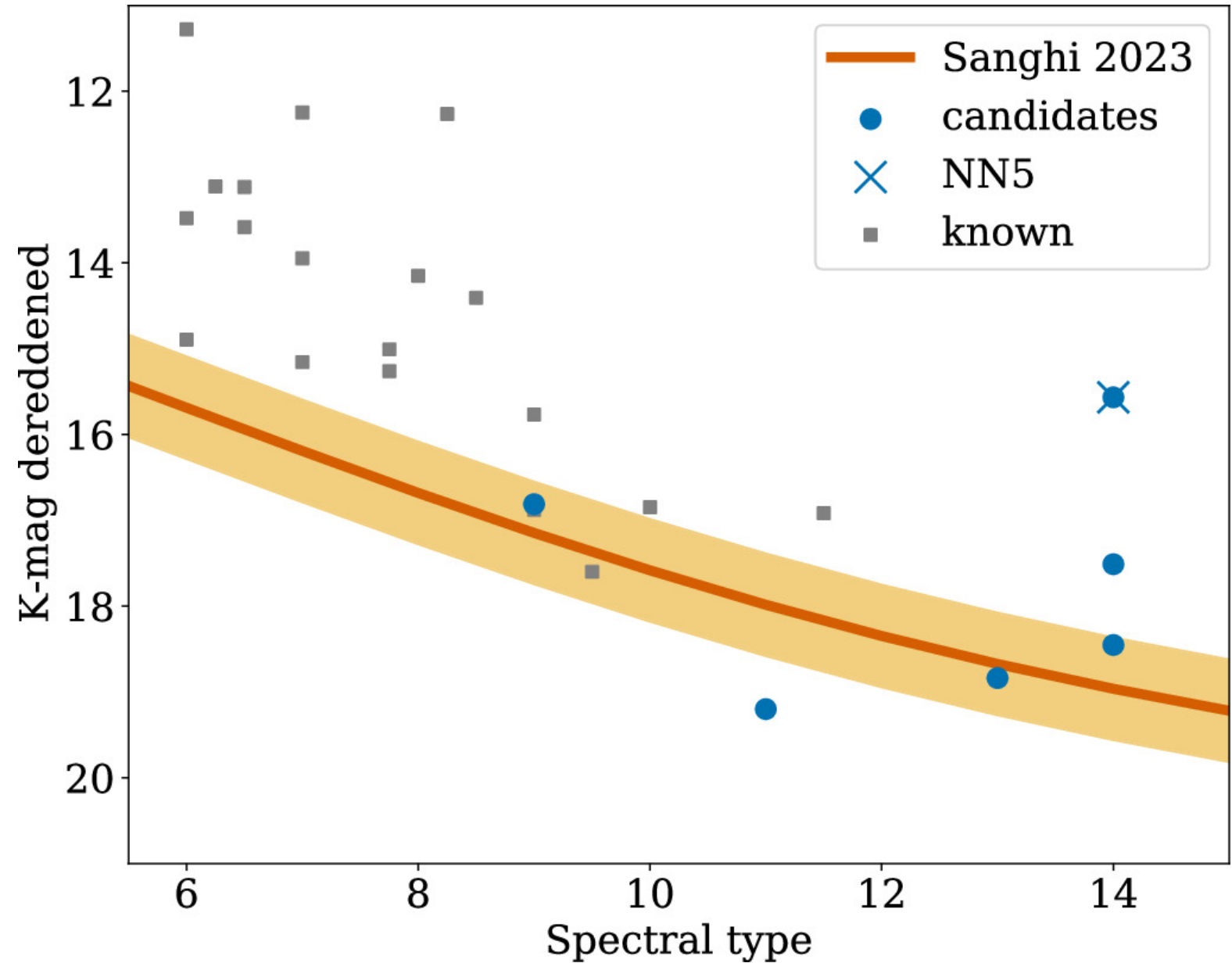
Figure 7. from Adam B. Langeveld et al 2024 Astron. J. 168 doi:10.3847/1538-3881/ad6f0c https://dx.doi.org/10.3847/1538-3881/ad6f0c © 2024. The Author(s). Published by the American Astronomical Society.
