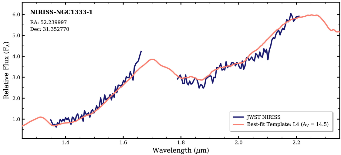
Figure 5. from Adam B. Langeveld et al 2024 Astron. J. 168 doi:10.3847/1538-3881/ad6f0c https://dx.doi.org/10.3847/1538-3881/ad6f0c © 2024. The Author(s). Published by the American Astronomical Society.
