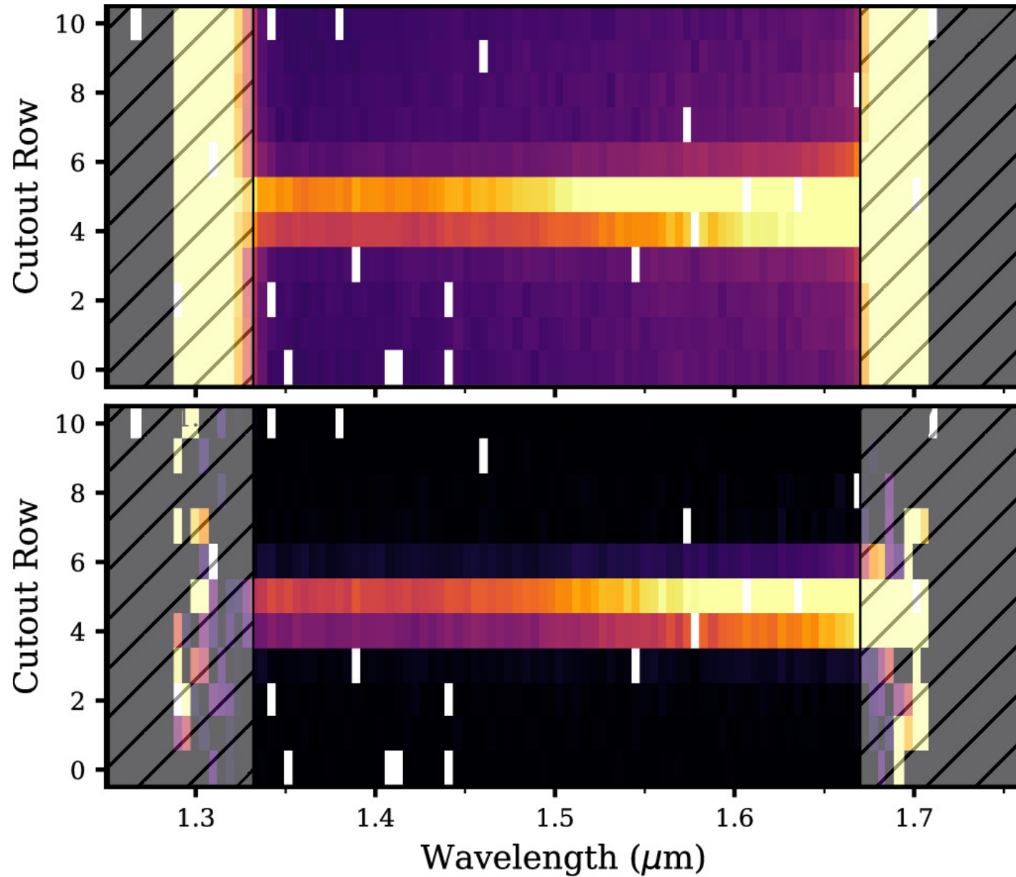
Figure 3. from Adam B. Langeveld et al 2024 Astron. J. 168 doi:10.3847/1538-3881/ad6f0c https://dx.doi.org/10.3847/1538-3881/ad6f0c © 2024. The Author(s). Published by the American Astronomical Society.
