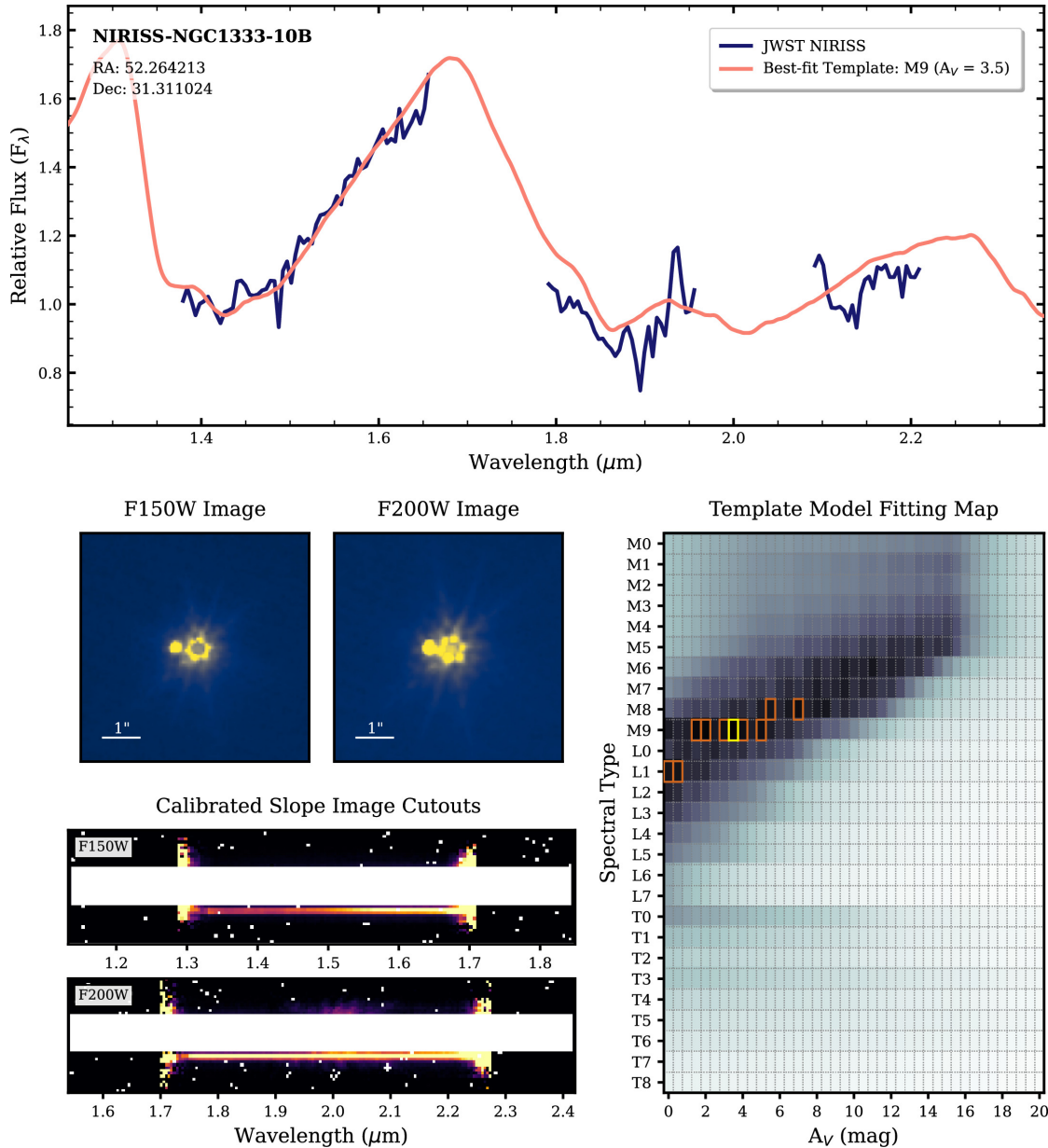
Figure 15. from Adam B. Langeveld et al 2024 Astron. J. 168 doi:10.3847/1538-3881/ad6f0c https://dx.doi.org/10.3847/1538-3881/ad6f0c © 2024. The Author(s). Published by the American Astronomical Society.
