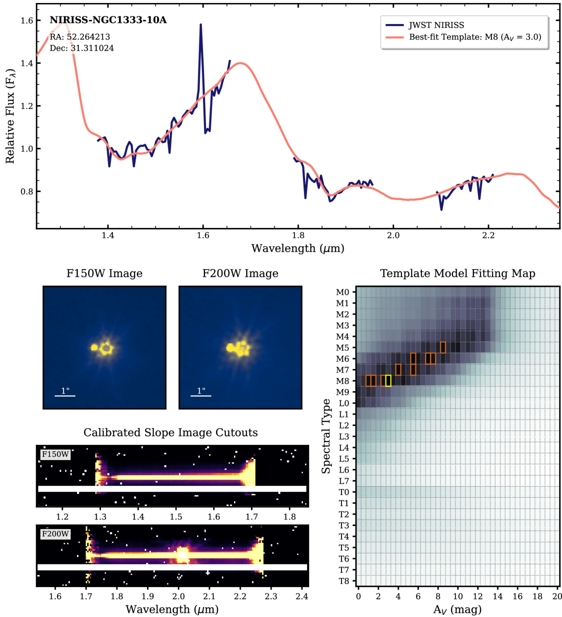
Figure 14. from Adam B. Langeveld et al 2024 Astron. J. 168 doi:10.3847/1538-3881/ad6f0c https://dx.doi.org/10.3847/1538-3881/ad6f0c © 2024. The Author(s). Published by the American Astronomical Society.
