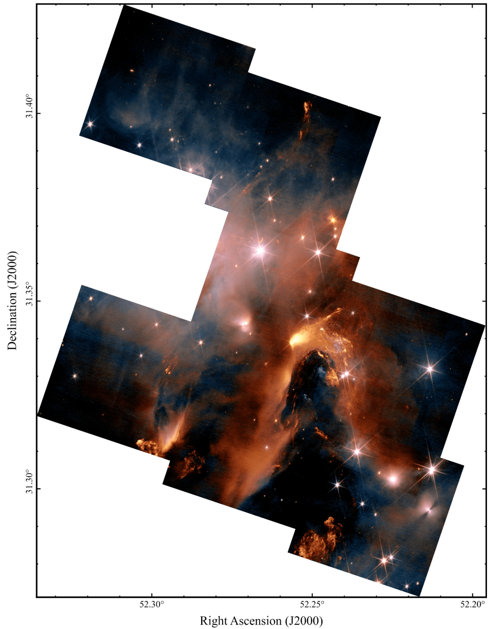
Figure 1. from Adam B. Langeveld et al 2024 Astron. J. 168 doi:10.3847/1538-3881/ad6f0c https://dx.doi.org/10.3847/1538-3881/ad6f0c © 2024. The Author(s). Published by the American Astronomical Society.
