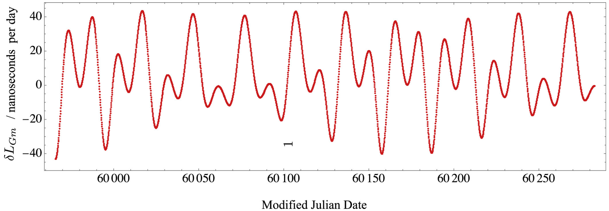
Figure 3. from Neil Ashby and Bijunath R. Patla 2024 Astron. J. 168 doi:10.3847/1538-3881/ad643a https://dx.doi.org/10.3847/1538-3881/ad643a © 2024. The Author(s). Published by the American Astronomical Society.
