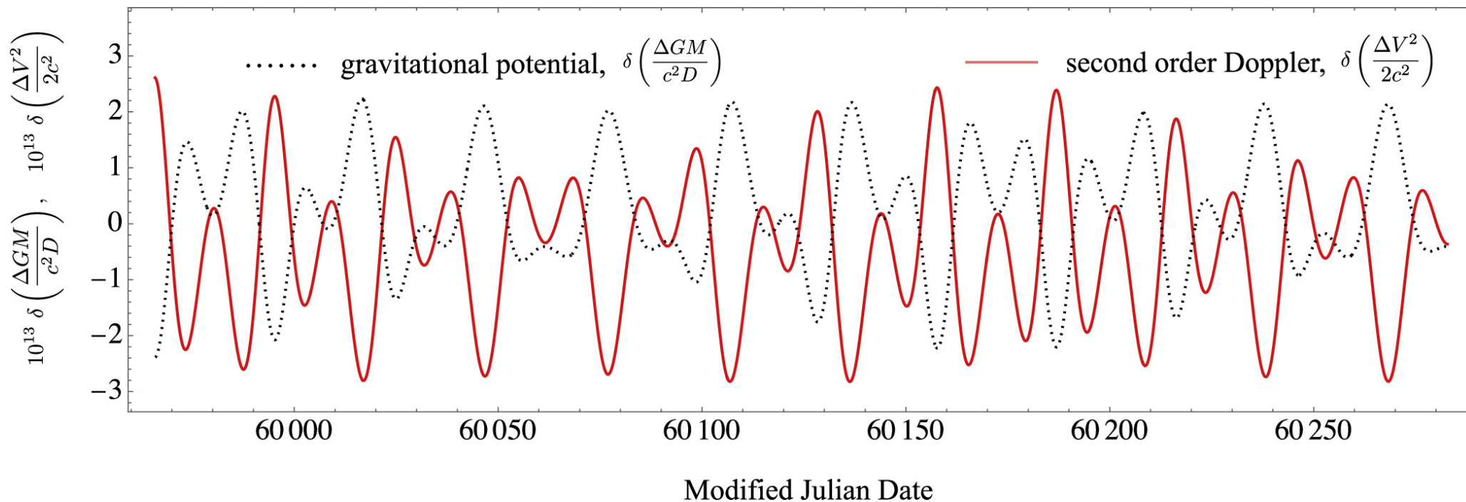
Figure 1. from Neil Ashby and Bijunath R. Patla 2024 Astron. J. 168 doi:10.3847/1538-3881/ad643a https://dx.doi.org/10.3847/1538-3881/ad643a © 2024. The Author(s). Published by the American Astronomical Society.
