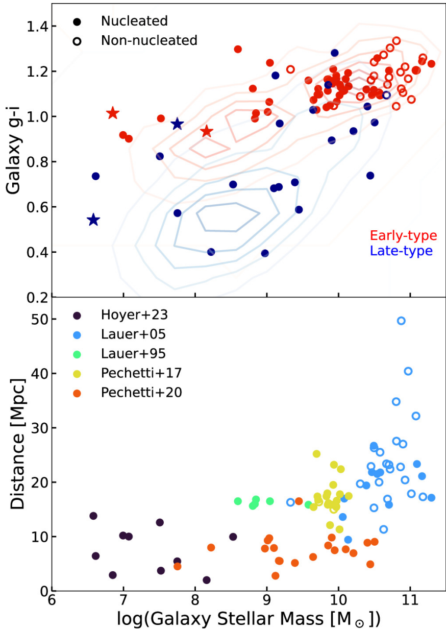
Figure 1. from Christian H. Hannah et al 2024 Astron. J. 168 doi:10.3847/1538-3881/ad630a https://dx.doi.org/10.3847/1538-3881/ad630a © 2024. The Author(s). Published by the American Astronomical Society.
