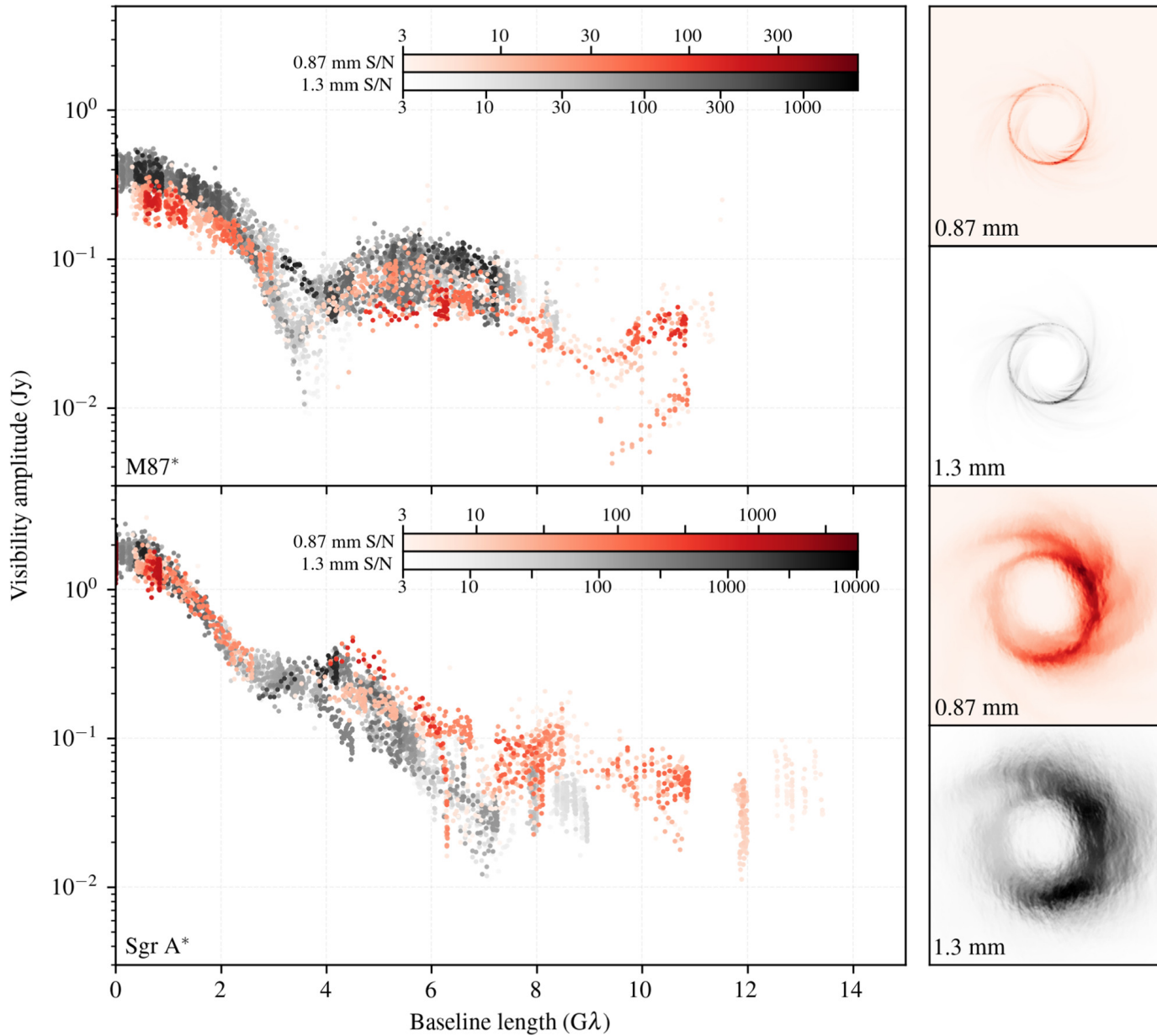
Figure 9. from Alexander W. Raymond et al 2024 Astron. J. 168 doi:10.3847/1538-3881/ad5bdb https://dx.doi.org/10.3847/1538-3881/ad5bdb © 2024. The Author(s). Published by the American Astronomical Society.
