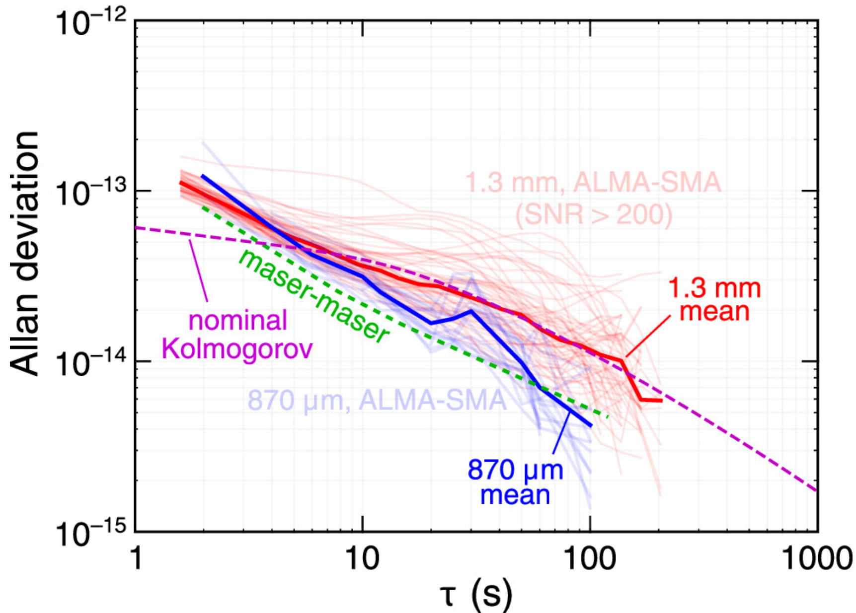
Figure 8. from Alexander W. Raymond et al 2024 Astron. J. 168 doi:10.3847/1538-3881/ad5bdb https://dx.doi.org/10.3847/1538-3881/ad5bdb © 2024. The Author(s). Published by the American Astronomical Society.
