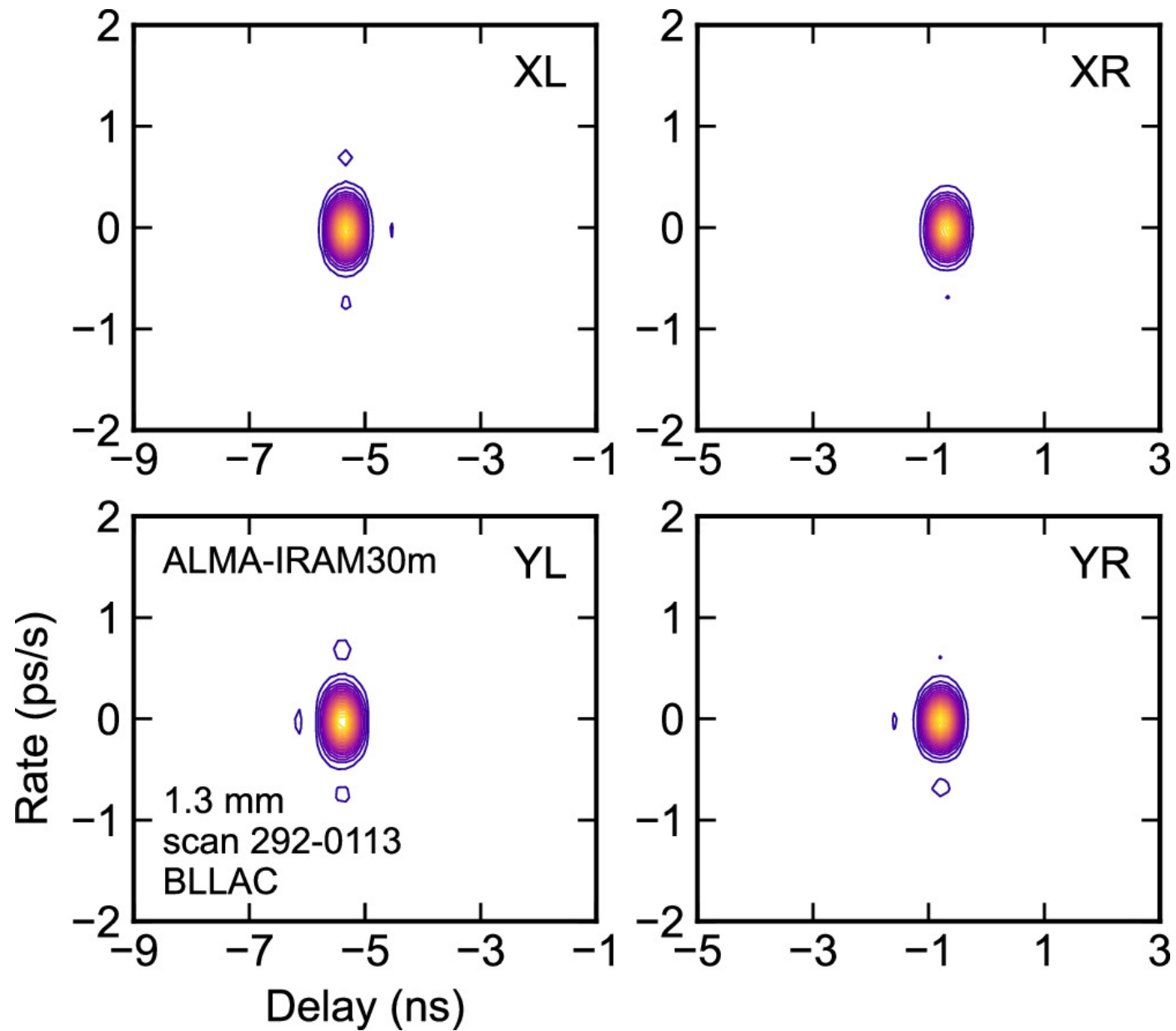
Figure 7. from Alexander W. Raymond et al 2024 Astron. J. 168 doi:10.3847/1538-3881/ad5bdb https://dx.doi.org/10.3847/1538-3881/ad5bdb © 2024. The Author(s). Published by the American Astronomical Society.
