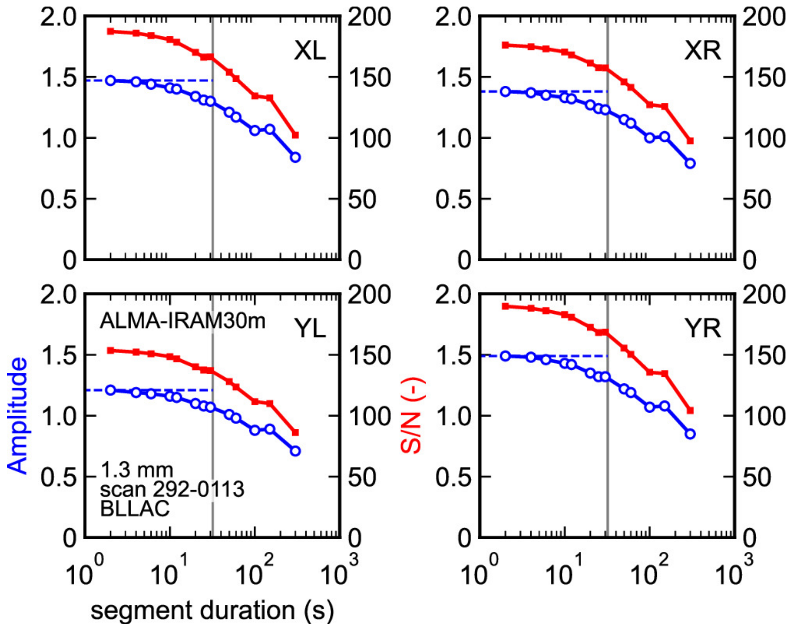
Figure 6. from Alexander W. Raymond et al 2024 Astron. J. 168 doi:10.3847/1538-3881/ad5bdb https://dx.doi.org/10.3847/1538-3881/ad5bdb © 2024. The Author(s). Published by the American Astronomical Society.
