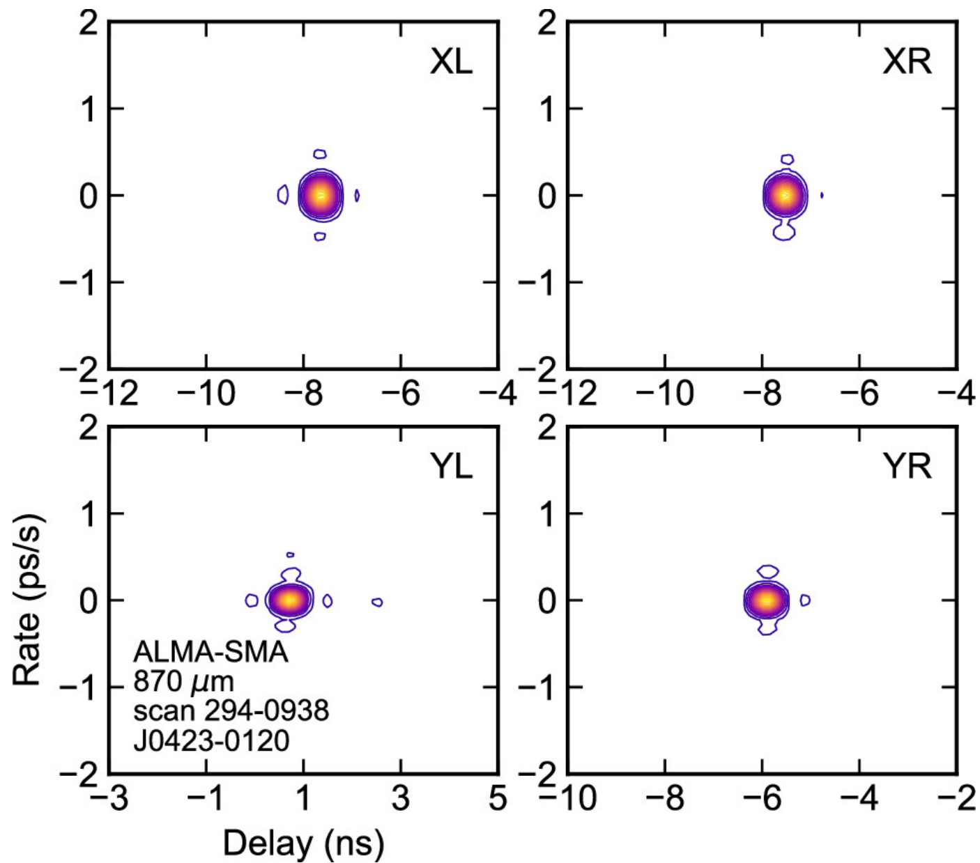
Figure 4. from Alexander W. Raymond et al 2024 Astron. J. 168 doi:10.3847/1538-3881/ad5bdb https://dx.doi.org/10.3847/1538-3881/ad5bdb © 2024. The Author(s). Published by the American Astronomical Society.
