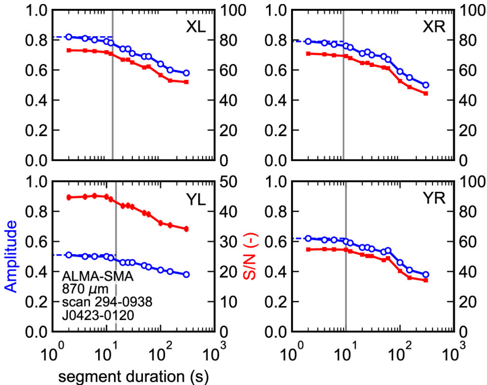
Figure 3. from Alexander W. Raymond et al 2024 Astron. J. 168 doi:10.3847/1538-3881/ad5bdb https://dx.doi.org/10.3847/1538-3881/ad5bdb © 2024. The Author(s). Published by the American Astronomical Society.
