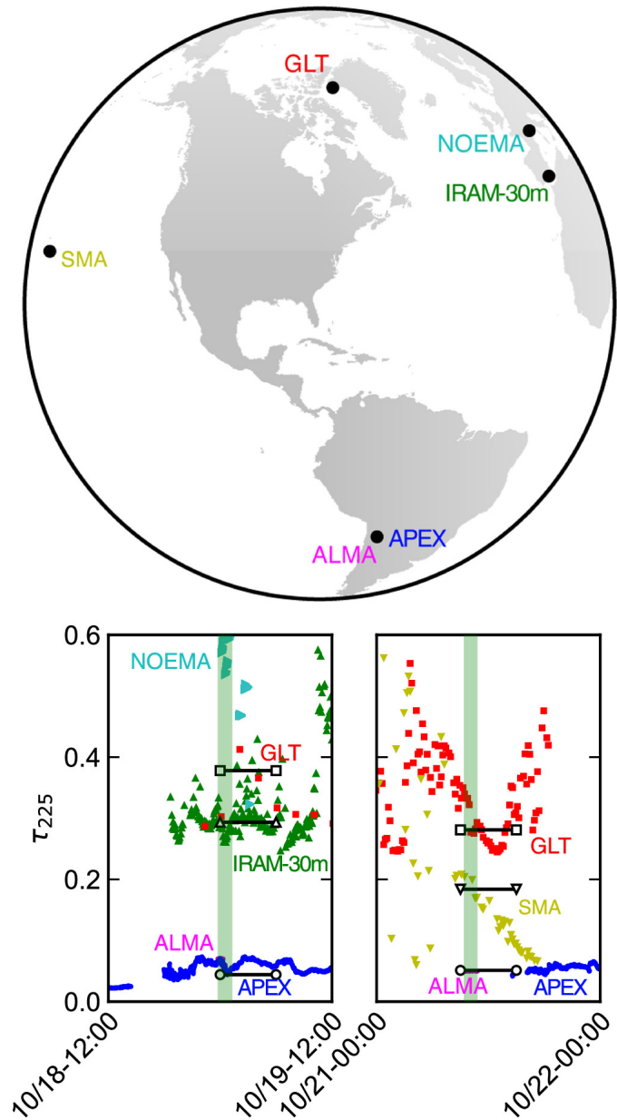
Figure 1. from Alexander W. Raymond et al 2024 Astron. J. 168 doi:10.3847/1538-3881/ad5bdb https://dx.doi.org/10.3847/1538-3881/ad5bdb © 2024. The Author(s). Published by the American Astronomical Society.
