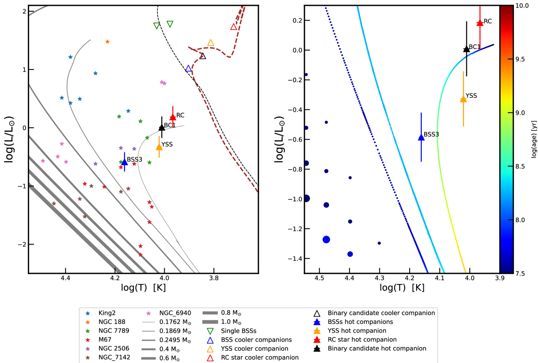
Figure 7. from Pinapati Saketh et al 2024 Astron. J. 168 doi:10.3847/1538-3881/ad5a96 https://dx.doi.org/10.3847/1538-3881/ad5a96 © 2024. The Author(s). Published by the American Astronomical Society.
