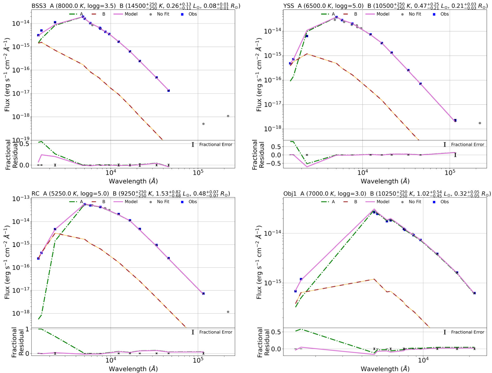
Figure 6. from Pinapati Saketh et al 2024 Astron. J. 168 doi:10.3847/1538-3881/ad5a96 https://dx.doi.org/10.3847/1538-3881/ad5a96 © 2024. The Author(s). Published by the American Astronomical Society.
